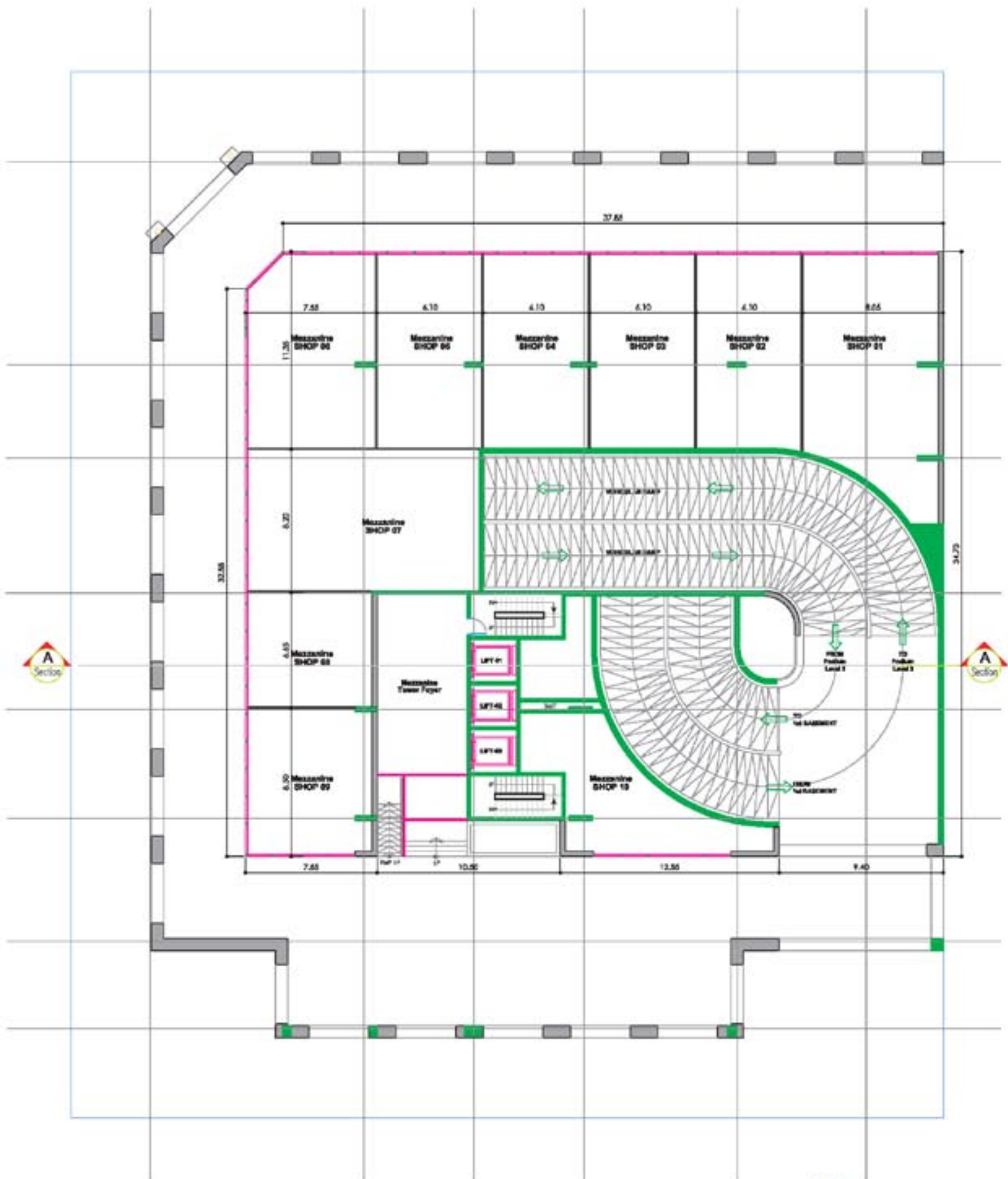
First Floor Retail Units (Mezzanine)
