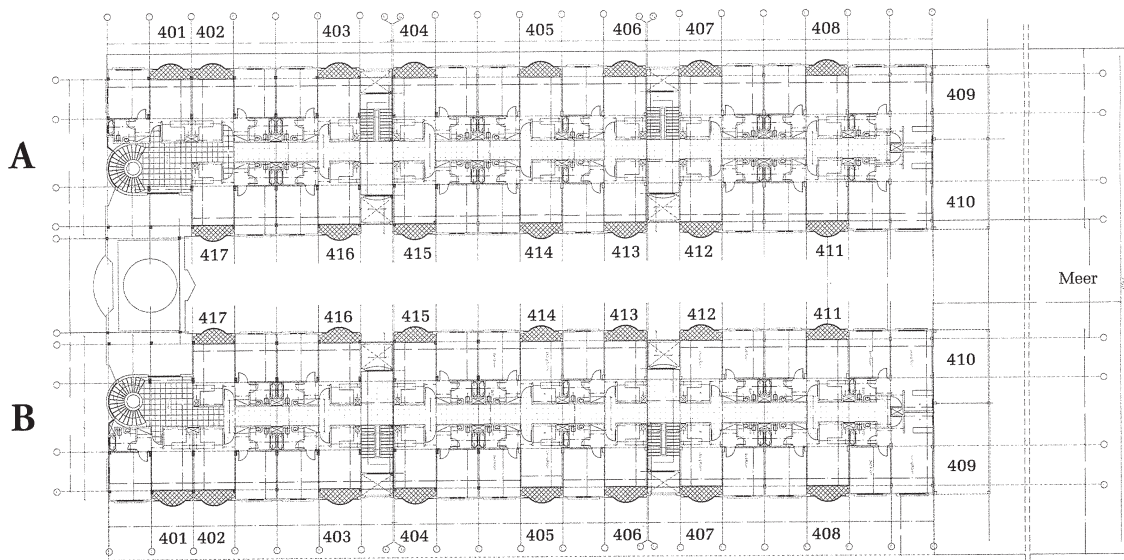
4th level building plan
