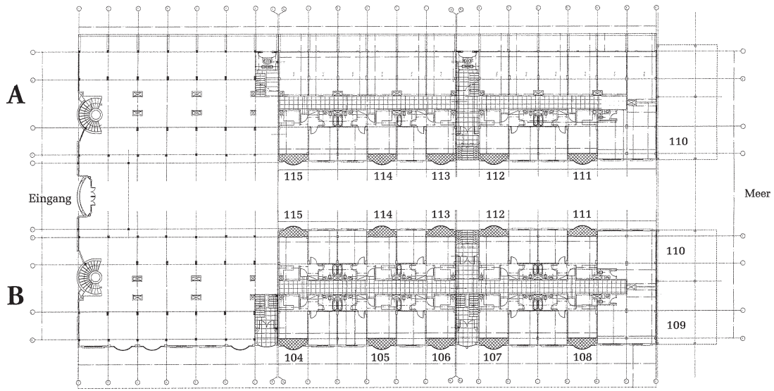
1st level building plan
