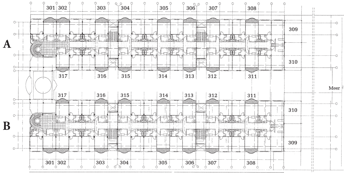
3rd level building plan
